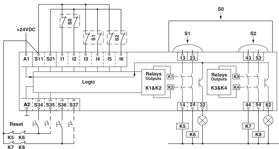
Circuit diagram
