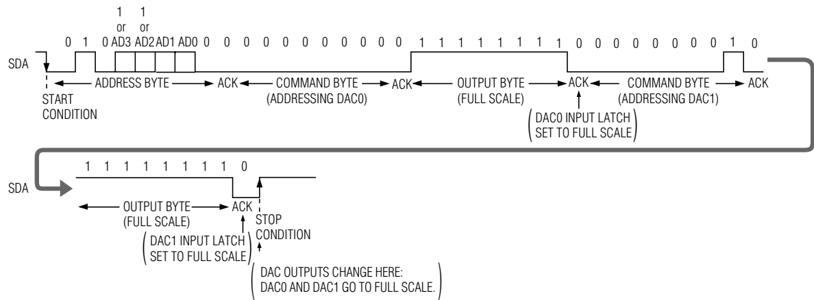
Figure 8b. Setting Both DAC Outputs (MAX518/MAX519)
