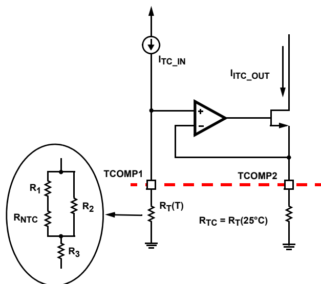
FIGURE 5. AVERAGE CURRENT TEMPERATURE COMPENSATION
