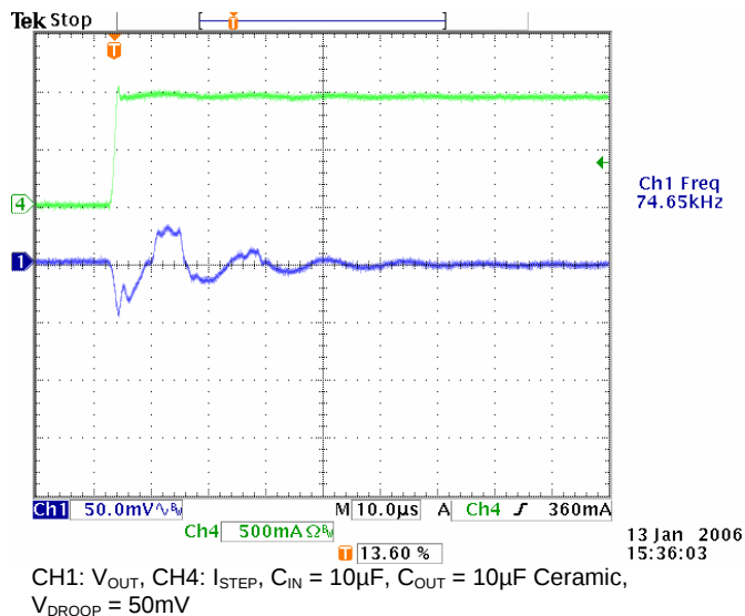
STEP LOAD STABILITY 10mA TO 1.0A
