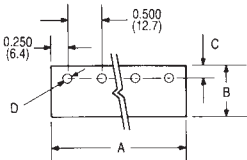
DUAL TO-220
