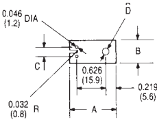
TO-66 (RECTANGLE)
