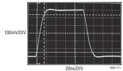
Figure 11. Step Response with R_F = 499\text{k}
