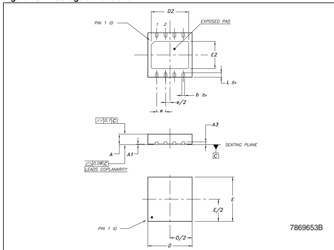
Figure 18. Package dimensions
