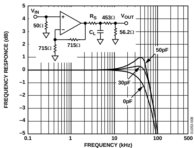
Figure 8. Frequency Response vs. Capacitive Load; C_L = 0\text{ pF} and 50\text{ pF} ; R_S = 0\text{ }\Omega
