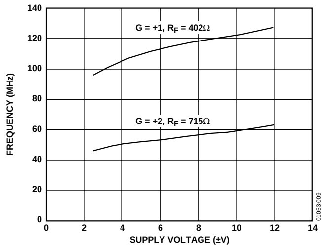
Figure 9. Bandwidth vs. Supply, R_L = 500\text{ }\Omega , V_{IN} = 200\text{ mV p-p}
