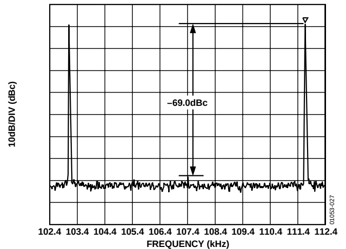
Figure 27. Multitone Power Ratio: V_S = \pm 6\text{ V} , R_L = 500\ \Omega , Full Rate ADSL (DMT), Upstream
