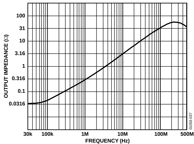
Figure 37. Output Impedance vs. Frequency, V_S = \pm 12 V
