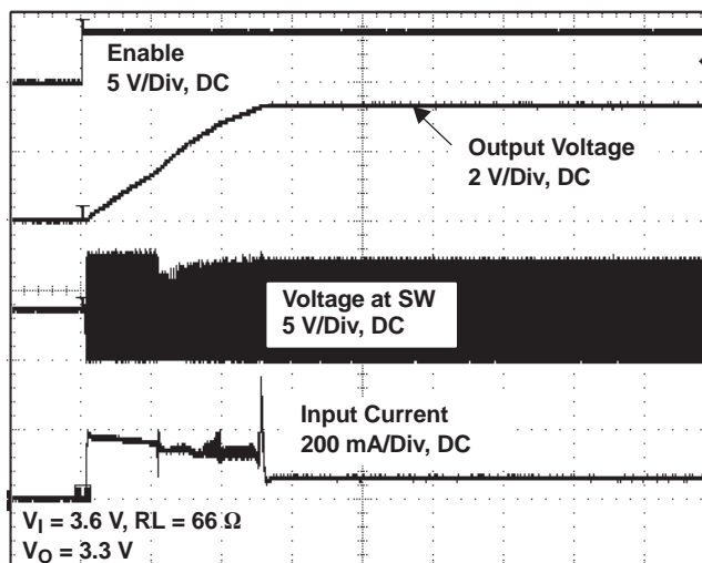
TPS61132 SEPIC CONVERTER START-UP AFTER ENABLE
