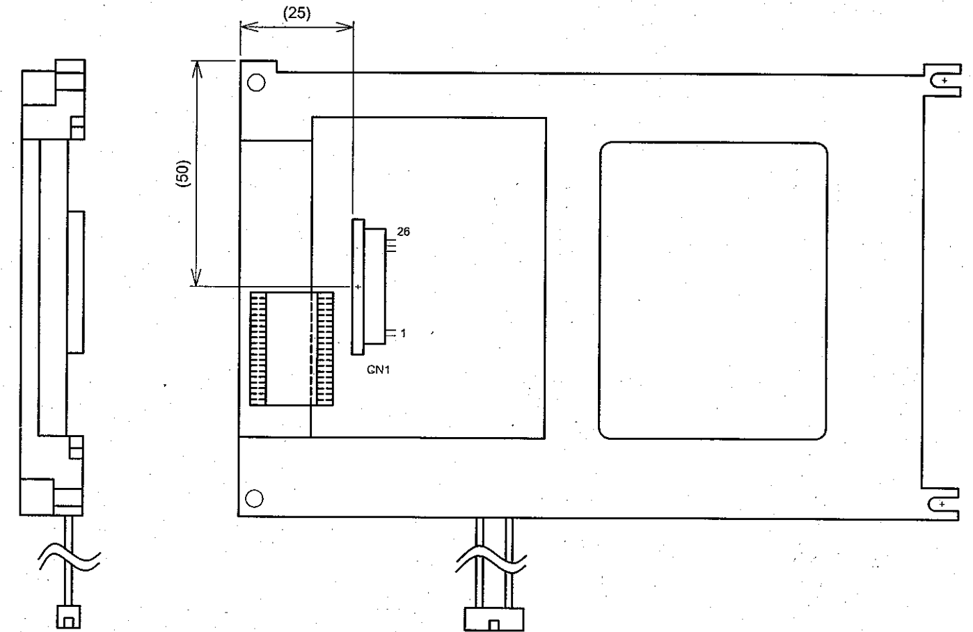
Rear View
