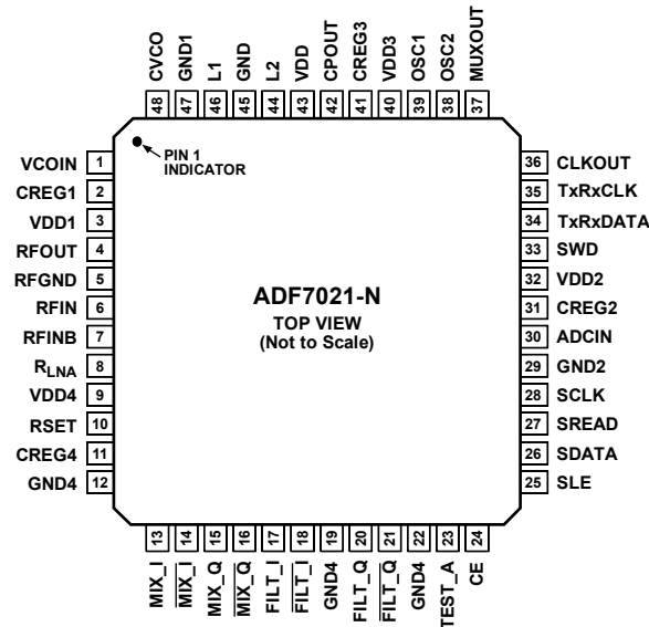
Figure 10. Pin Configuration
