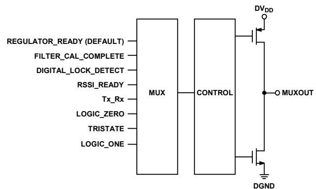
Figure 36. MUXOUT Circuit
