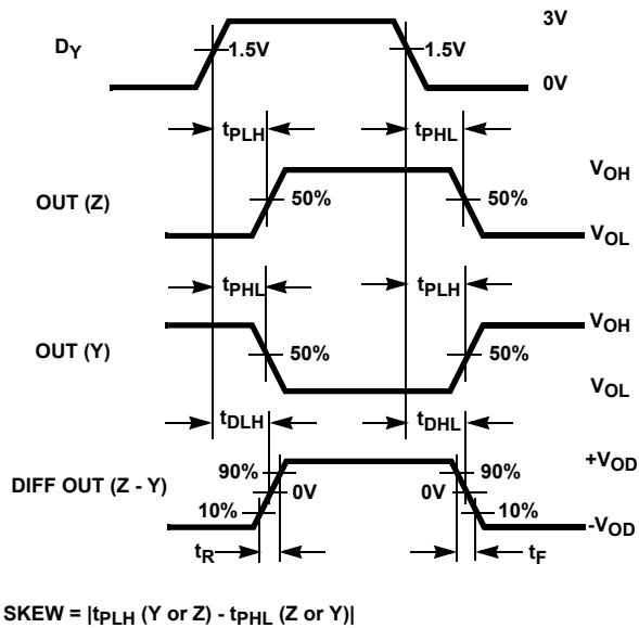
FIGURE 10B. MEASUREMENT POINTS
