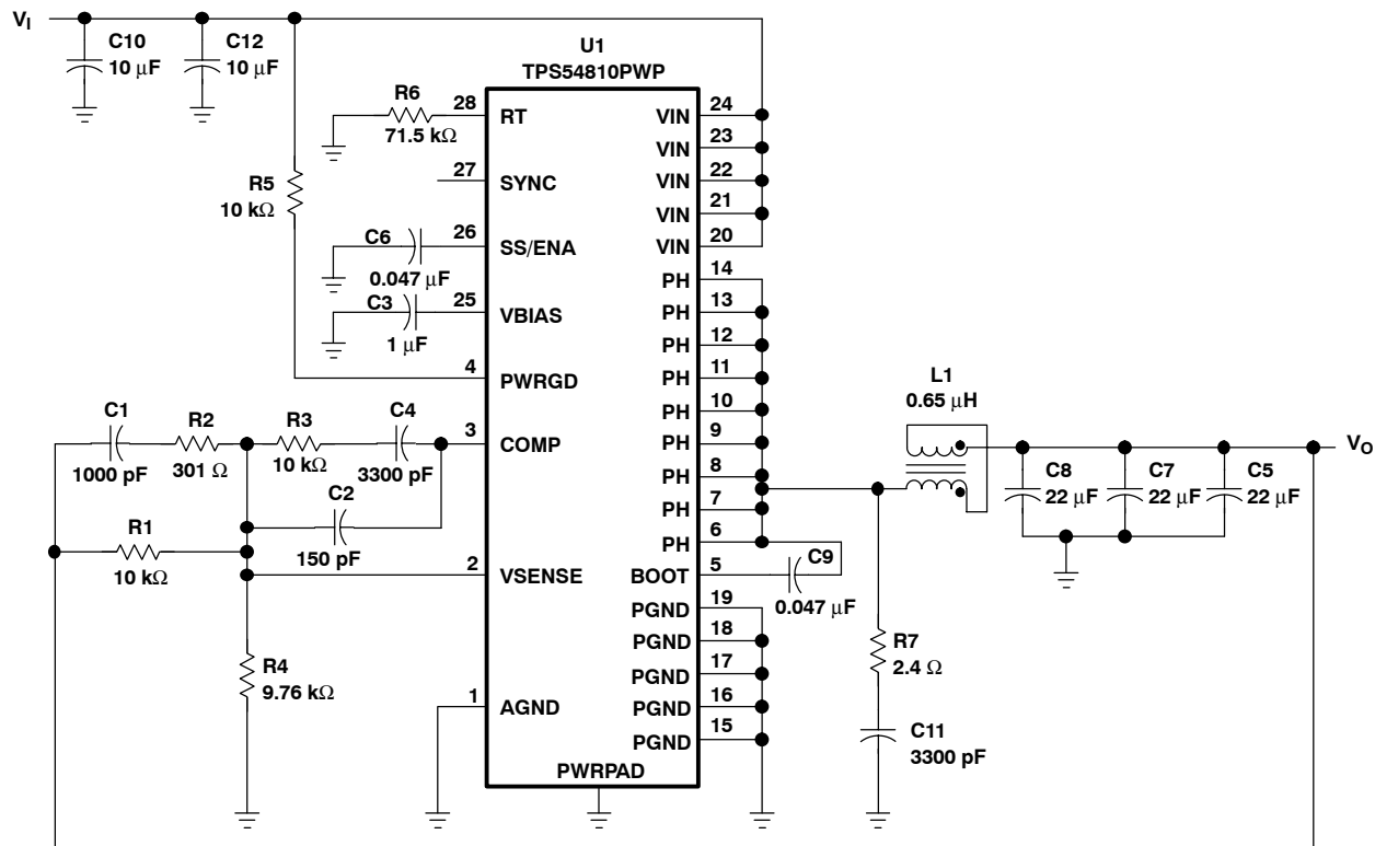
Figure 9. Application Circuit
