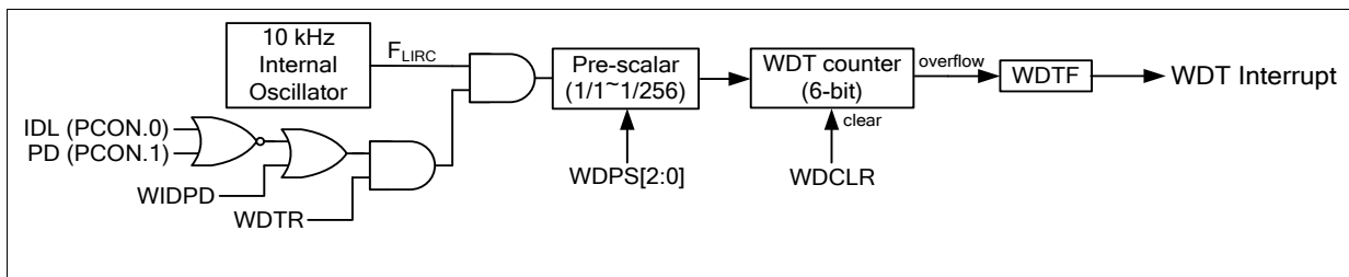
Figure 11.2. Watchdog Timer Block Diagram
