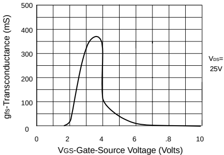
Transconductance v gate-source voltage
