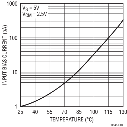
Input Bias vs Temperature
