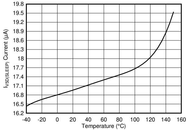
Figure 6-7. VSD Sleep Current vs Temperature
