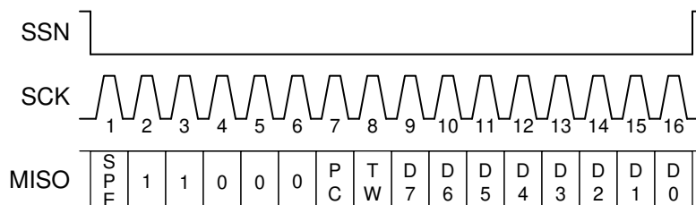
Figure 7-17. Read Response Frame Format
