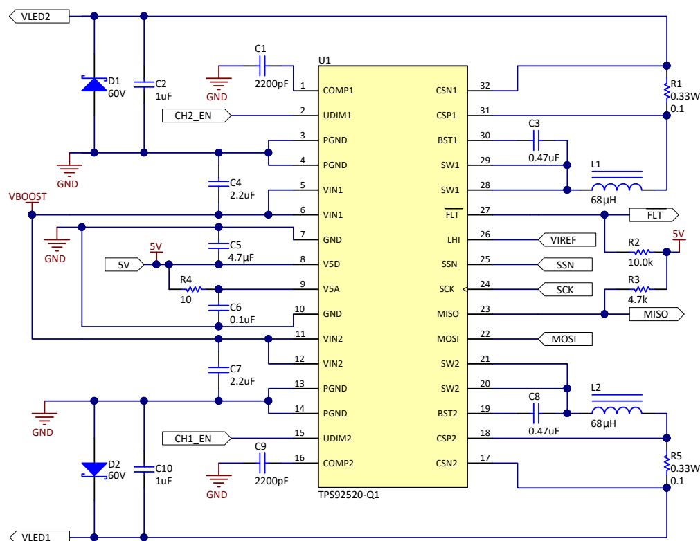
Figure 8-3. Application Schematic
