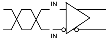
Figure 7. Differential Inputs Driven Differentially
