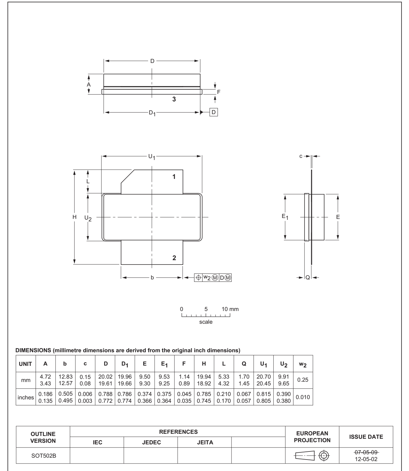
Fig 9. Package outline SOT502B
