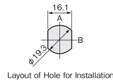
Layout of Hole for Installation
