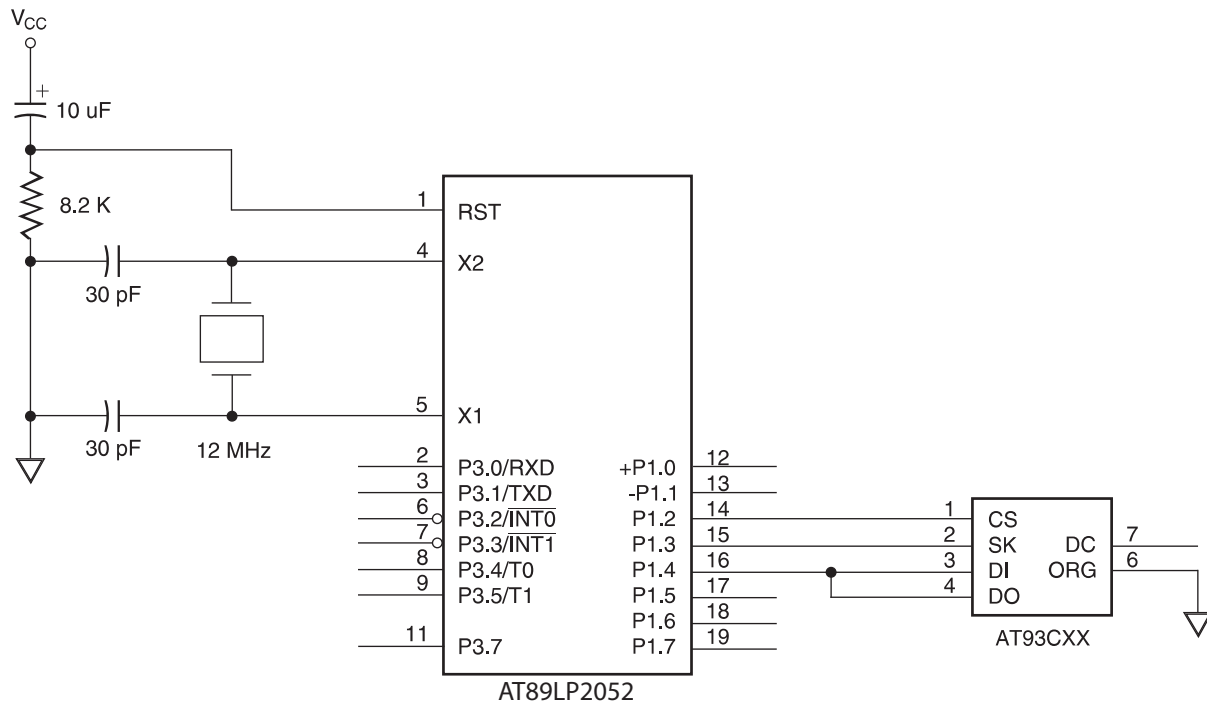
Figure 1-1. 3-Wire Configuration
