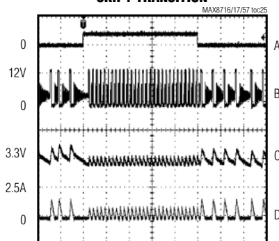
SKIP1 TRANSITION
