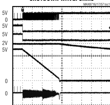
SHUTDOWN WAVEFORMS
