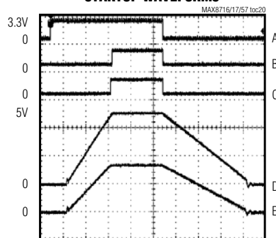
STARTUP WAVEFORMS
