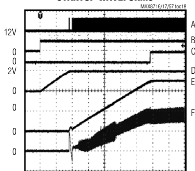
STARTUP WAVEFORMS
