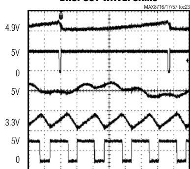
DROPOUT WAVEFORMS
