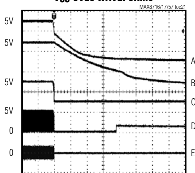
V CC UVLO WAVEFORMS
