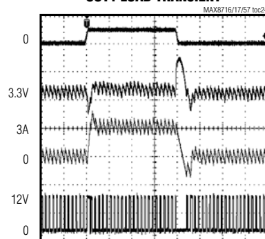
OUT1 LOAD TRANSIENT
