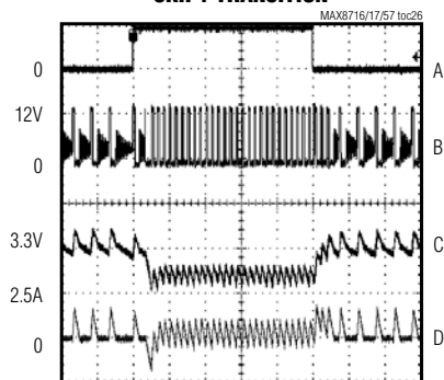
SKIP1 TRANSITION
