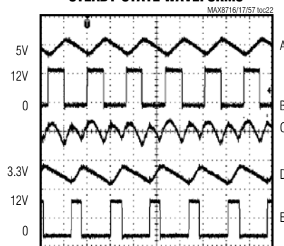
STEADY-STATE WAVEFORMS
