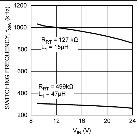
Figure 4. Switching Frequency, f_{SW} vs V_{IN}
