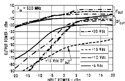
Limiting Characteristics
