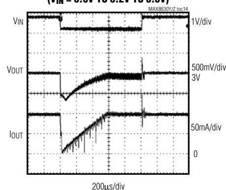
LINE-TRANSIENT RESPONSE WITH MODE CHANGE ( V_{IN} = 3.8V TO 3.2V TO 3.8V )
