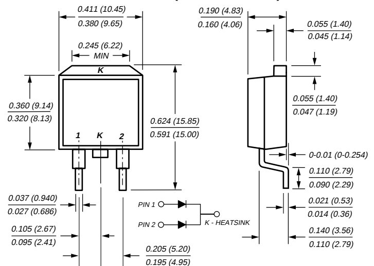
TO-263AB (BYVB32 Series)
