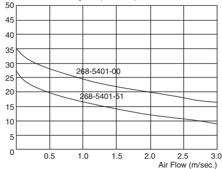
Thermal Resistance \Theta J-A ( ^{\circ} C WATT)
