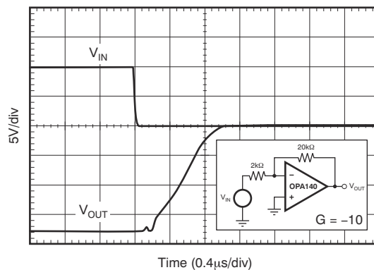
Figure 6-24. Negative Overload Recovery
