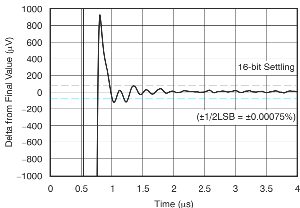
Figure 6-24. Negative Overload Recovery
