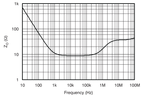
Figure 6-18. Open-Loop Output Impedance vs Frequency
