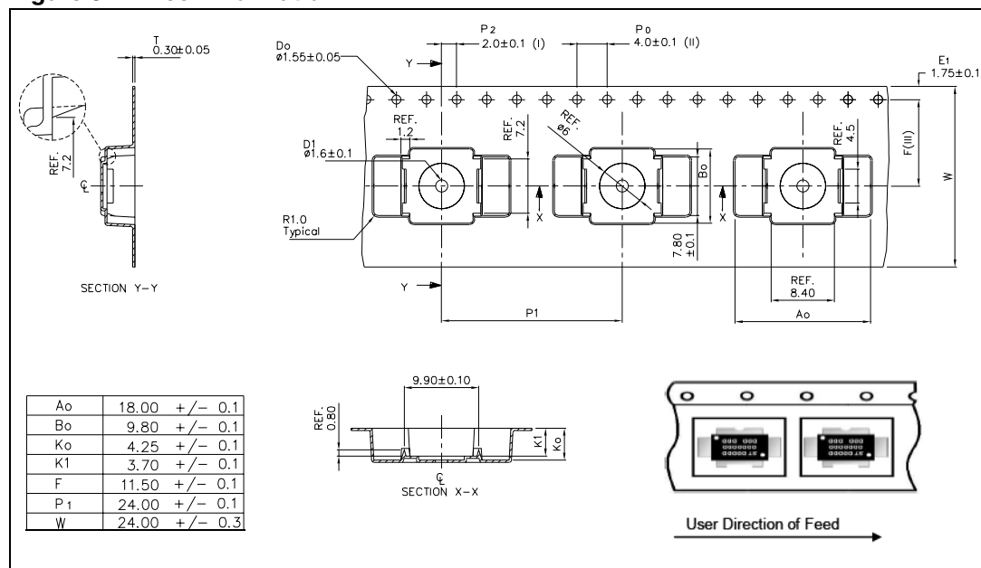
Figure 31. Reel information
