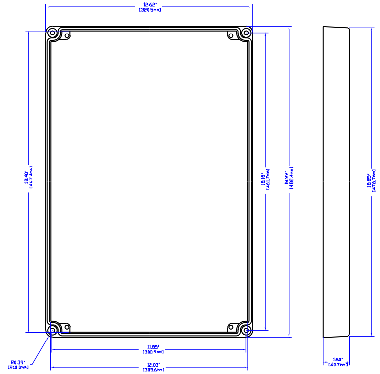
VIEW OF LID (INSIDE)
