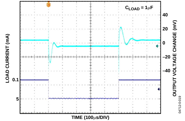
Figure 19. Regulator Load Transient Response
