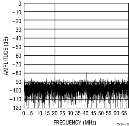
LTC2234: 8192 Point FFT, f_{IN} = 250\text{MHz} , -1dB, 1V Range
