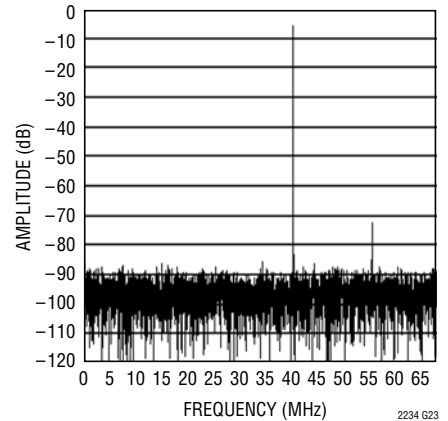
LTC2234: 8192 Point FFT, f_{IN} = 500\text{MHz} , -6dB, 1V Range
