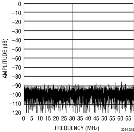
LTC2234: 8192 Point FFT, f_{IN} = 30\text{MHz} , -1dB, 2V Range
