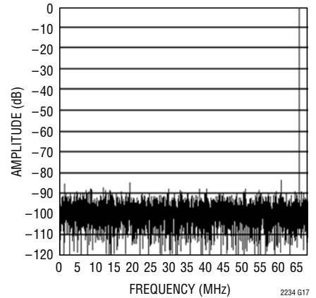
LTC2234: 8192 Point FFT, f_{IN} = 70\text{MHz} , -1dB, 2V Range
