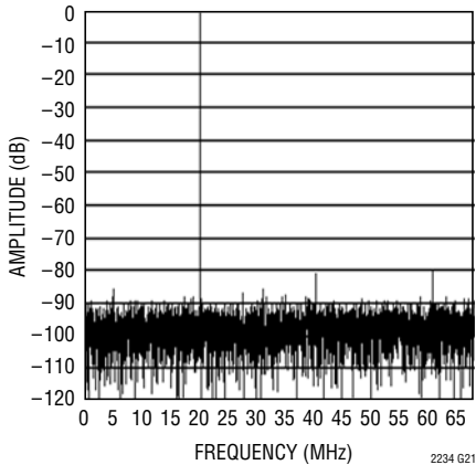
LTC2234: 8192 Point FFT, f_{IN} = 250\text{MHz} , -1dB, 2V Range
