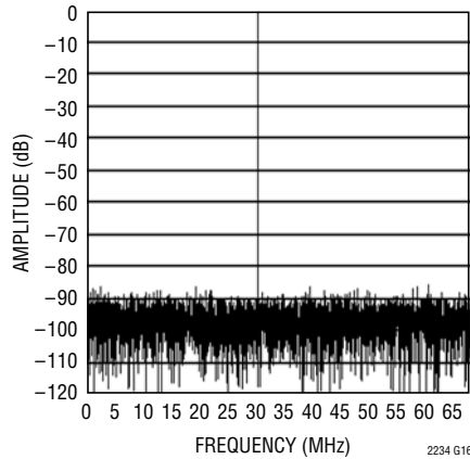
LTC2234: 8192 Point FFT, f_{IN} = 30\text{MHz} , -1dB, 1V Range
