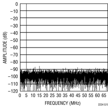
LTC2234: 8192 Point FFT, f_{IN} = 140\text{MHz} , -1dB, 2V Range
