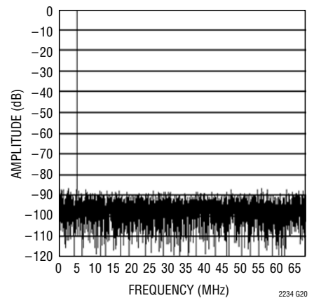
LTC2234: 8192 Point FFT, f_{IN} = 140\text{MHz} , -1dB, 1V Range
