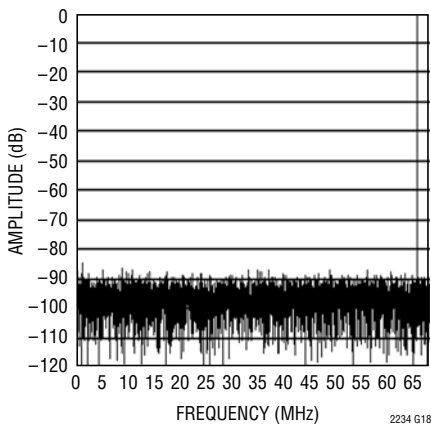
LTC2234: 8192 Point FFT, f_{IN} = 70\text{MHz} , -1dB, 1V Range
