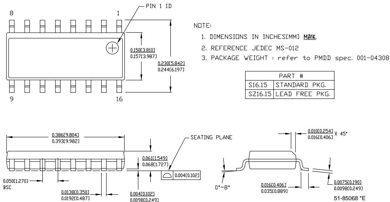
Figure 15. 16-Pin (150-Mil) SOIC
