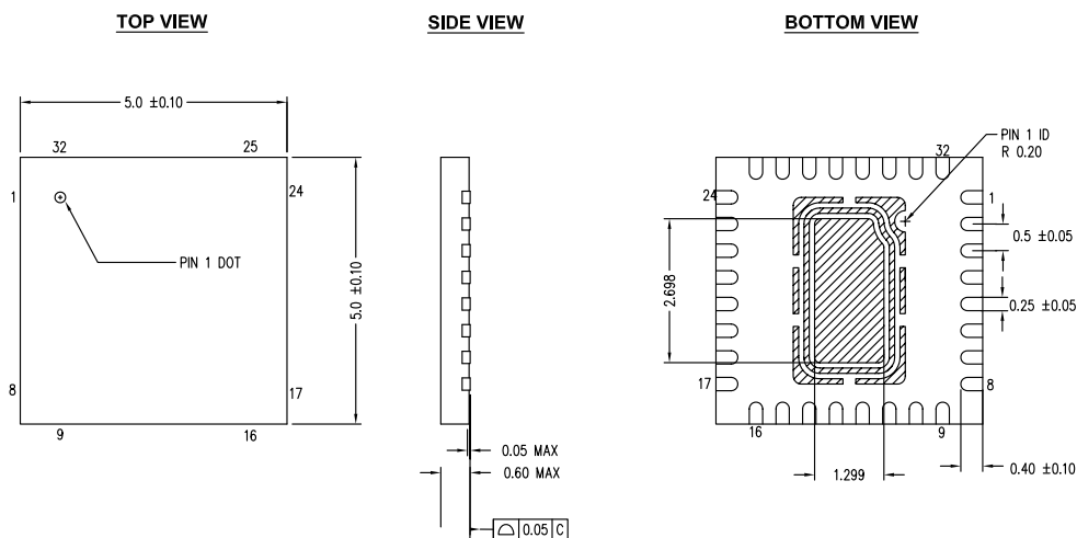
Figure 20. 32-pin QFN (5 × 5 × 0.55 mm) 1.3 × 2.7 E-Pad (Sawn Type) Package Outline
