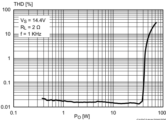
Figure 26. THD vs. output power ( V_S = 14.4\ V , R_L = 2\ \Omega )
