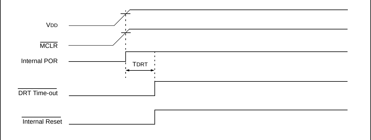
FIGURE 5-5: TIME-OUT SEQUENCE ON POWER-UP ( \overline{\text{MCLR}} TIED TO \text{V}_{\text{DD}} ): SLOW \text{V}_{\text{DD}} RISE TIME
