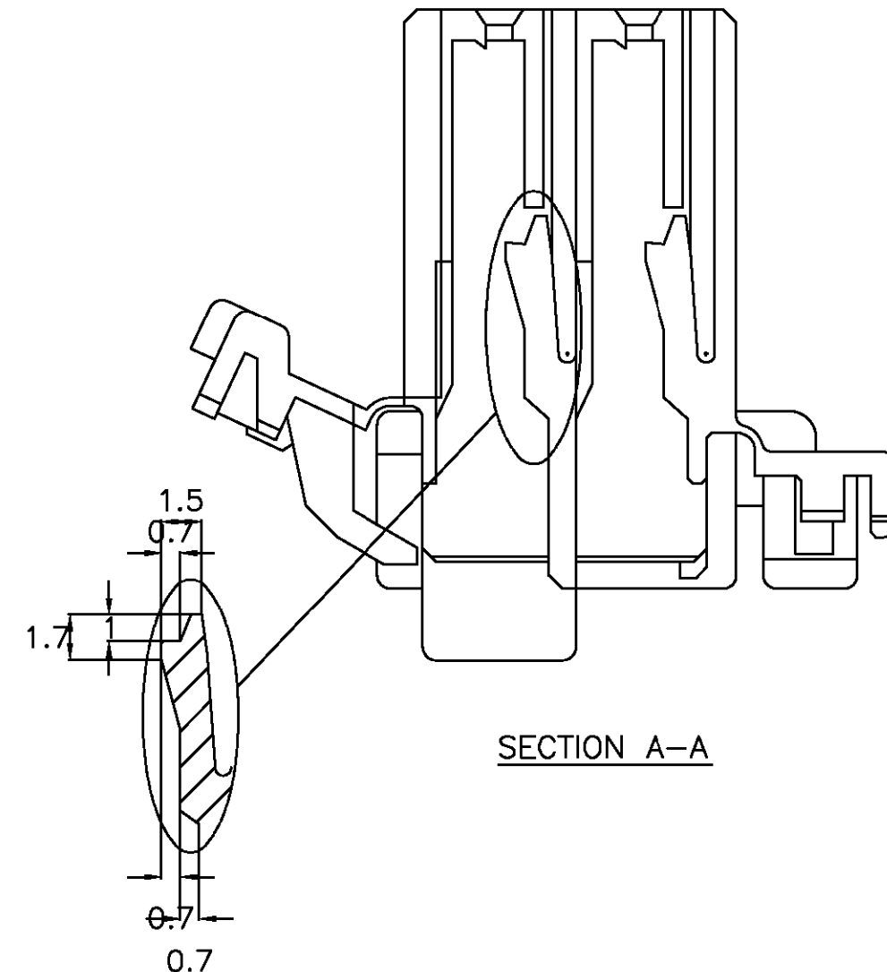
LANCE DETAIL
