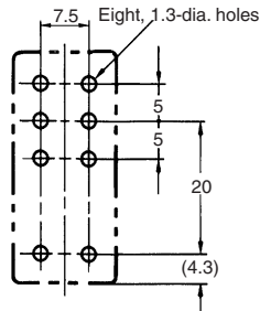
Mounting Holes
