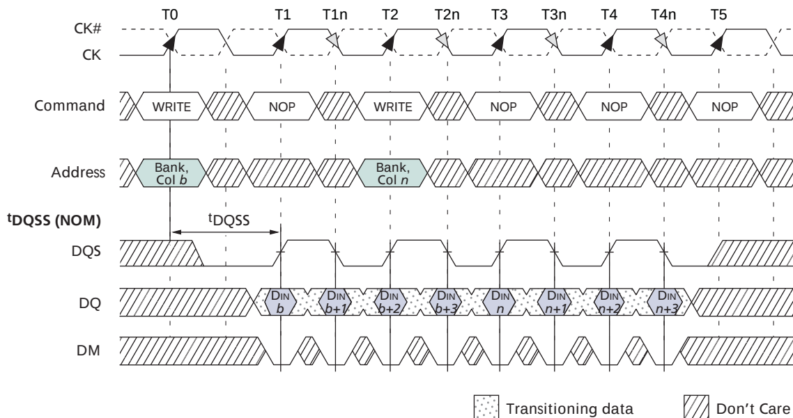
Figure 23: Consecutive WRITE-to-WRITE
