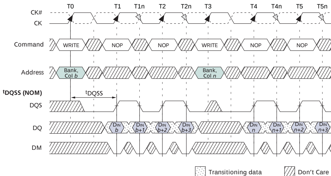
Figure 24: Nonconsecutive WRITE-to-WRITE
