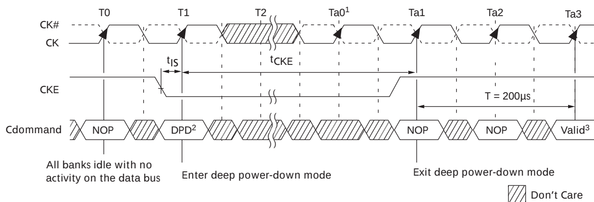
Figure 35: Deep Power-Down
