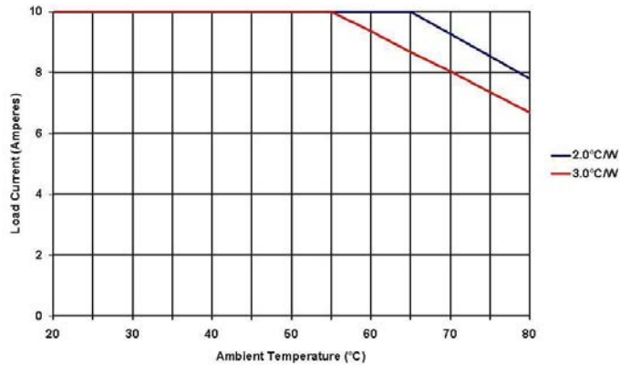
DERATING CURVE: 8413x860
