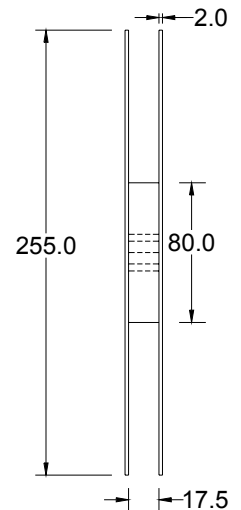
2k Reel Dimensions in mm
