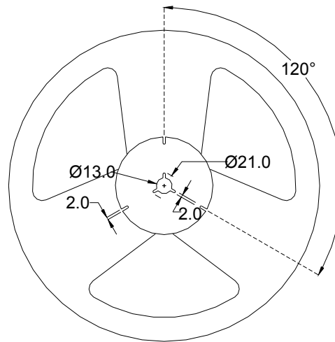
2k Reel Dimensions in mm
