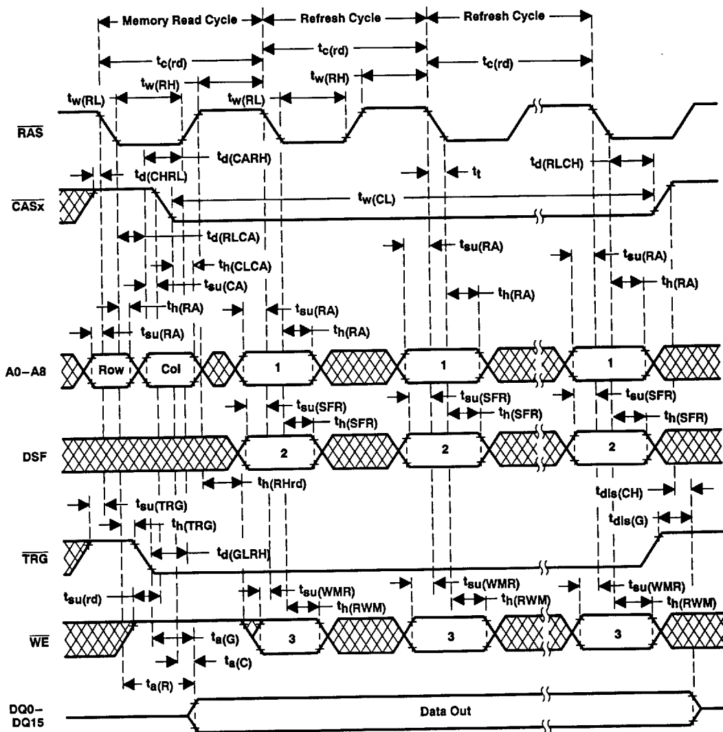
Figure 40. Hidden-Refresh-Cycle Timing
