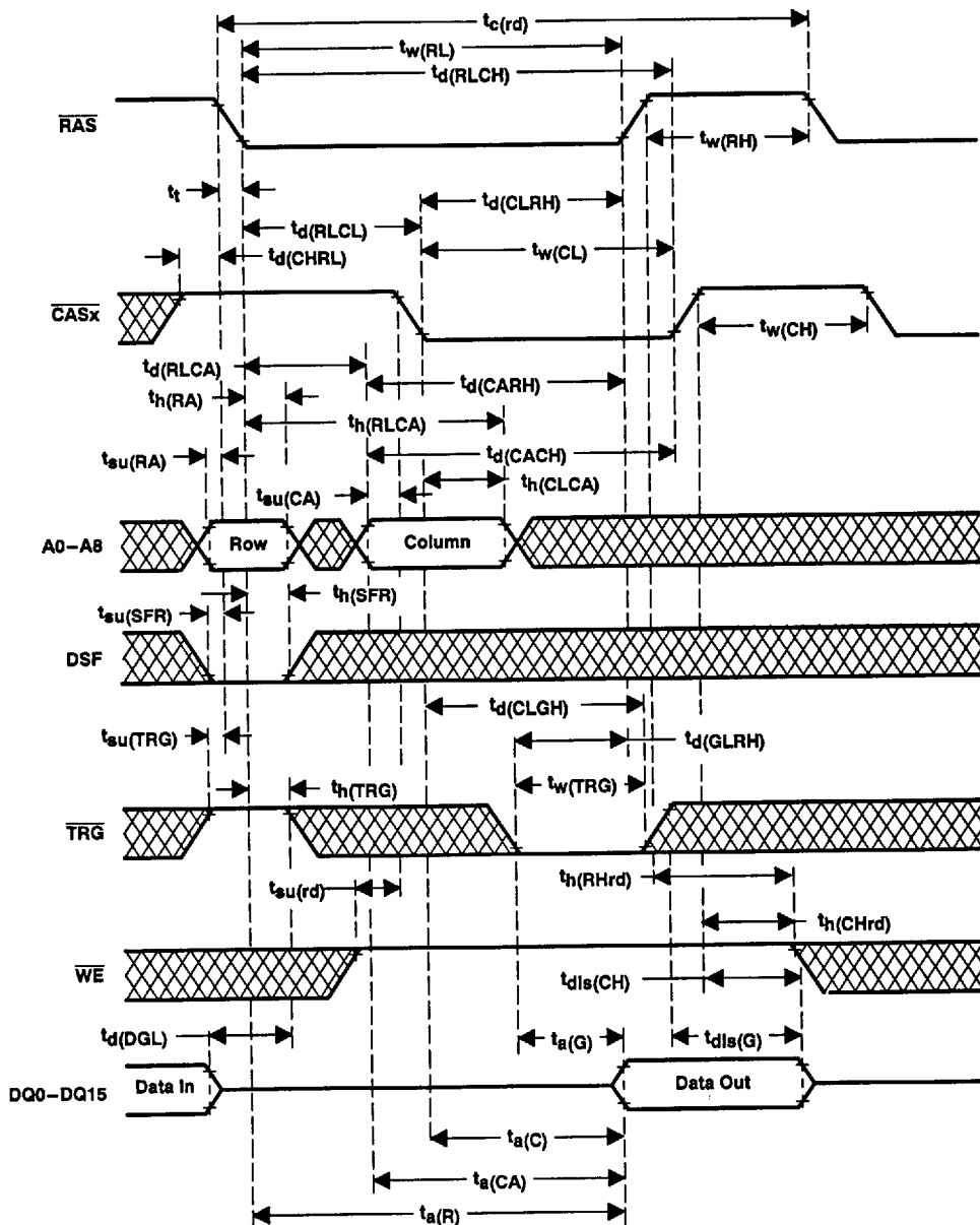
Figure 24. Read-Cycle Timing
