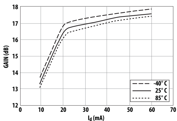
Figure 8. Gain vs. I_d and Temperature at 900 MHz.
