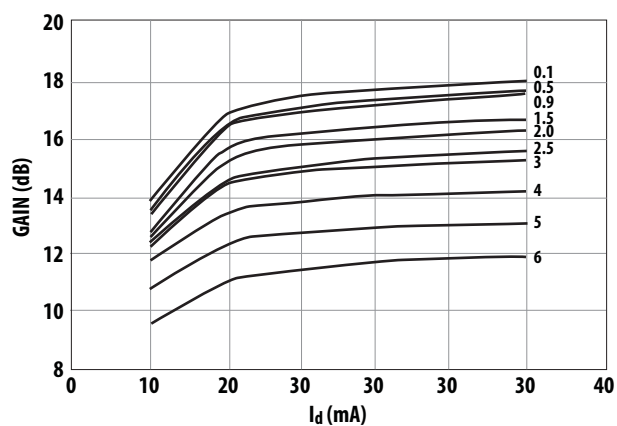
Figure 12. Gain vs. I d and Frequency (GHz).
