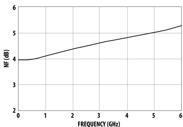
Figure 6. NF vs. Frequency at I_d = 35 mA.
