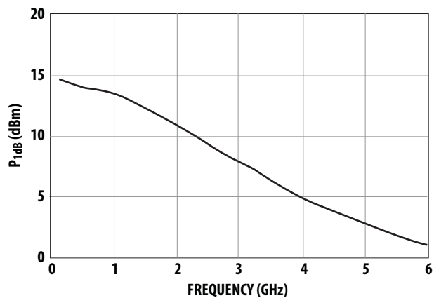
Figure 4. P_{1dB} vs. Frequency at I_d = 35 mA.
