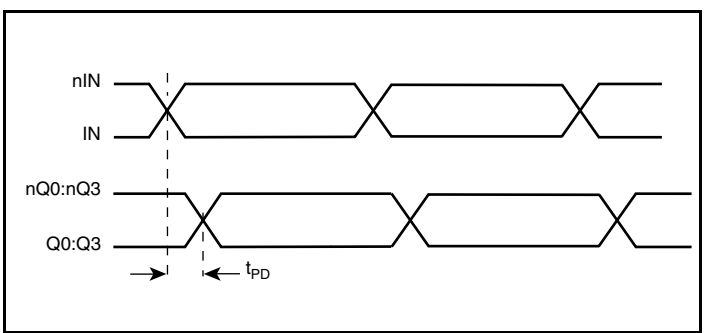
Propagation Delay
