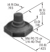
AT4054 Round Solid Colored Cap Polycarbonate Colors: BJ CJ EJ FJ GJ Series: LB Panel Seal
