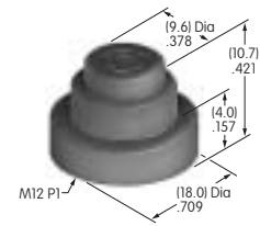
AT4055 Round Colored Insert Cap Polycarbonate Colors: JB JC JE JF JG Series: LB Panel Seal
