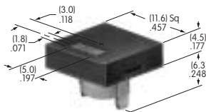
AT4051 Spot Illuminated Cap Polycarbonate Colors: AB Series: KB
