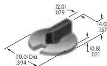
AT4061 Snap-in Knob Polyamide Knob Color: A Flange Color: J Series: DR
