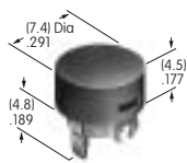
AT4036 Round Nonilluminated Cap Polycarbonate Colors: B C E F G Series: HB
