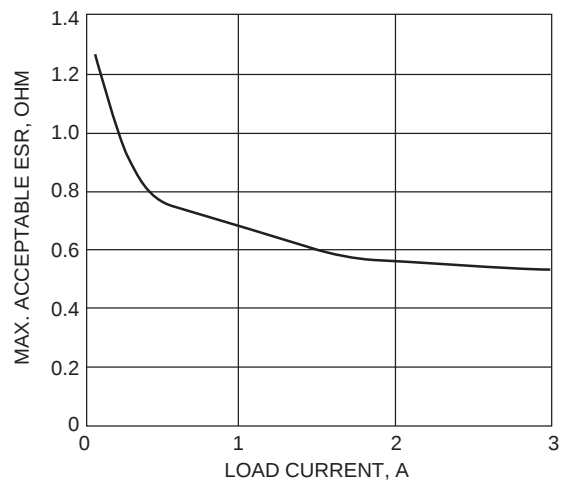
FAN1582 Stability
