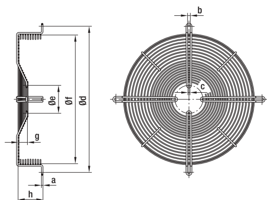
Basket guard grilles for S-Range axial fans
