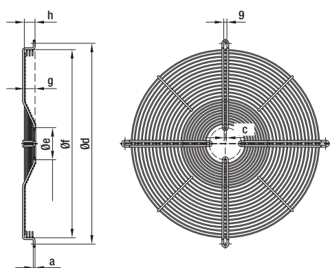
Basket guard grilles for S-Range axial fans (for mounting on square wall rings with long nozzle)
