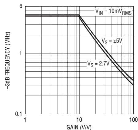
LTC6912-1 -3dB Bandwidth vs Gain Setting
