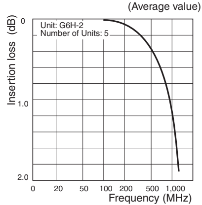
Frequency vs. Insertion Loss
