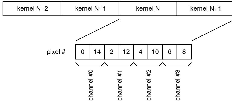
Figure 39. P1–SN/FN: Data Output Order for 4 LVDS Output Channels in Subsampling Mode on a Monochrome Sensor
