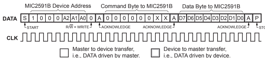
Figure 10. WRITE_BYTE Protocol
